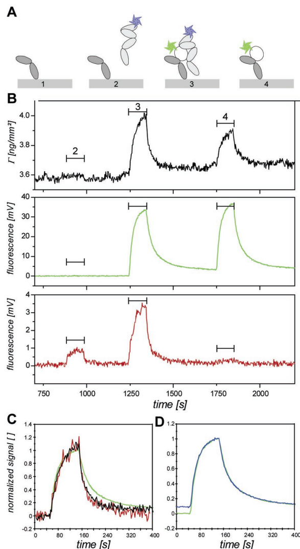
Figure 7. Dissection of multi-protein complex formation by surface-sensitive detection. (A) Schematic of the binding assays: after immobilization of ifnar2-H10 (1), first H10-ifnar1-labeled with ^{FEW646}\text{tris-NTA} was injected (2), then the complex of H10-ifnar1/ ^{FEW646}\text{tris-NTA} with ^{OG488}\text{IFN}\alpha 2 (3), and then ^{OG488}\text{IFN}\alpha 2 alone (4). (B) Typical binding curves as detected by simultaneous TIRFS-Rif detection upon sequential injection of 200 nM H10-ifnar1 with 800 nM ^{FEW646}\text{tris-NTA} (I), 200 nM H10-ifnar1 with 800 nM ^{FEW646}\text{tris-NTA} and 100 nM ^{OG488}\text{IFN}\alpha 2 (II), and 100 nM ^{OG488}\text{IFN}\alpha 2 (II): mass signal (black), green fluorescence (green), and red fluorescence (red). (C) Overlay of the three signals during injection II normalized to the maximum signal (same color coding as panel B). (D) Overlay of the green fluorescence signal during injection II (green) and injection III (blue), normalized to the maximum signal.
