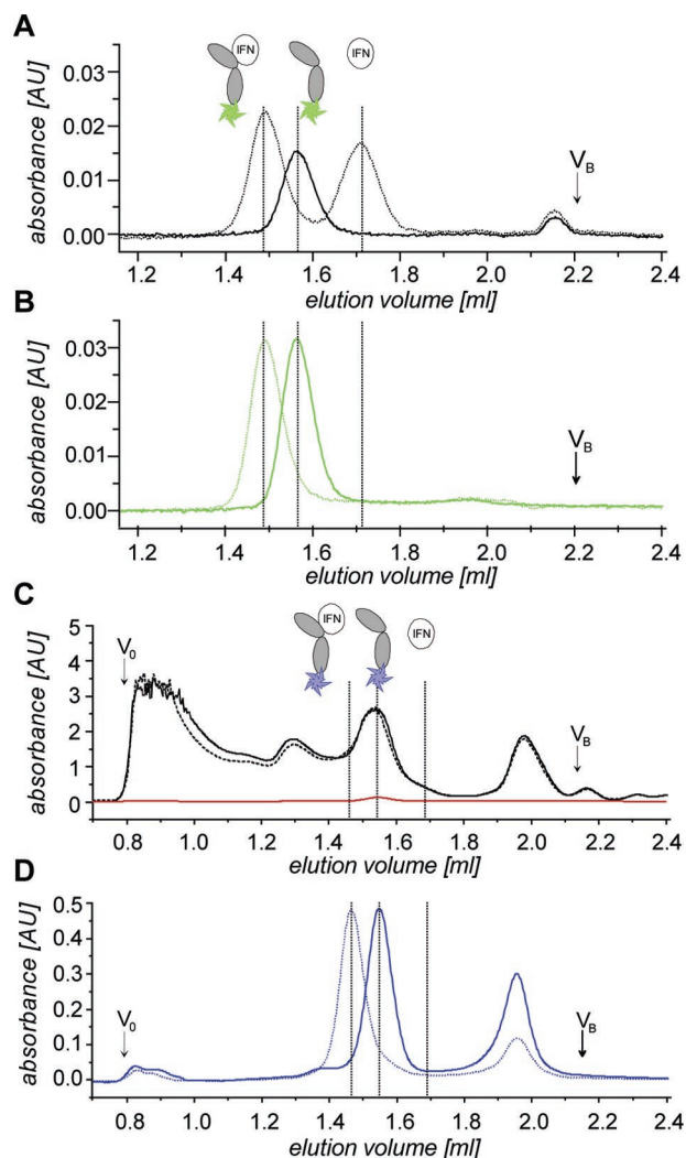
Figure 3. Site-specific and selective labeling of ifnar2-H10 by tris-NTA conjugates. (A and B) Analytical SEC of OG488 tris-NTA-labeled ifnar2-H10 (1 \mu M) after removing excess OG488 tris-NTA (—). The chromatograms were recorded simultaneously at 280 nm (A) and 490 nm (B). The same sample was incubated with 1.5 \mu M IFN \alpha 2 and chromatographed under the same conditions (.....). (C and D) FEW646 tris-NTA-Mediated labeling of ifnar2-H10 in a cell lysate analyzed by analytical SEC. A crude E. coli cell lysate (OD 280 ~400 AU) seeded with ifnar2-H10 (10 \mu M, OD 280 ~0.3 AU) was incubated with FEW646 tris-NTA (15 \mu M) and chromatographed with simultaneous detection at 280 nm (C) and 600 nm (D). When stoichiometric quantities of FEW646 tris-NTA were used, only one peak at 1.55 mL was observed (data not shown). The spectral characteristics of the signal detected in the exclusion volume suggested that it stemmed from scattering and not from nonspecifically bound fluorescence dye. The same experiment was carried out after adding 15 \mu M IFN \alpha 2 (.....).
