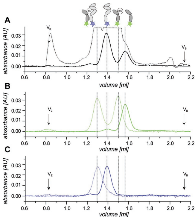
Figure 5. Ternary complex formation of ifnar2-EC and ifnar1-EC with IFN \beta as detected by analytical SEC. Ifnar2-H10 and ifnar1-H10 were labeled with OG488-tris-NTA and FEW646-tris-NTA, respectively. OG488-tris-NTA-labeled ifnar2-H10 and FEW646-tris-NTA-labeled ifnar1-H10 were mixed, and SEC was carried out with detection at 280 nm (A), 490 nm (B), and 600 nm (C) before (.....) and after (—) the addition of IFN \beta . The dotted lines mark the elution volumes of ifnar2-H10, of the IFN \beta /ifnar2-H10 complex, of ifnar1-H10, and of the ternary complex between ifnar1-H10, ifnar2-H10, and IFN \beta .
