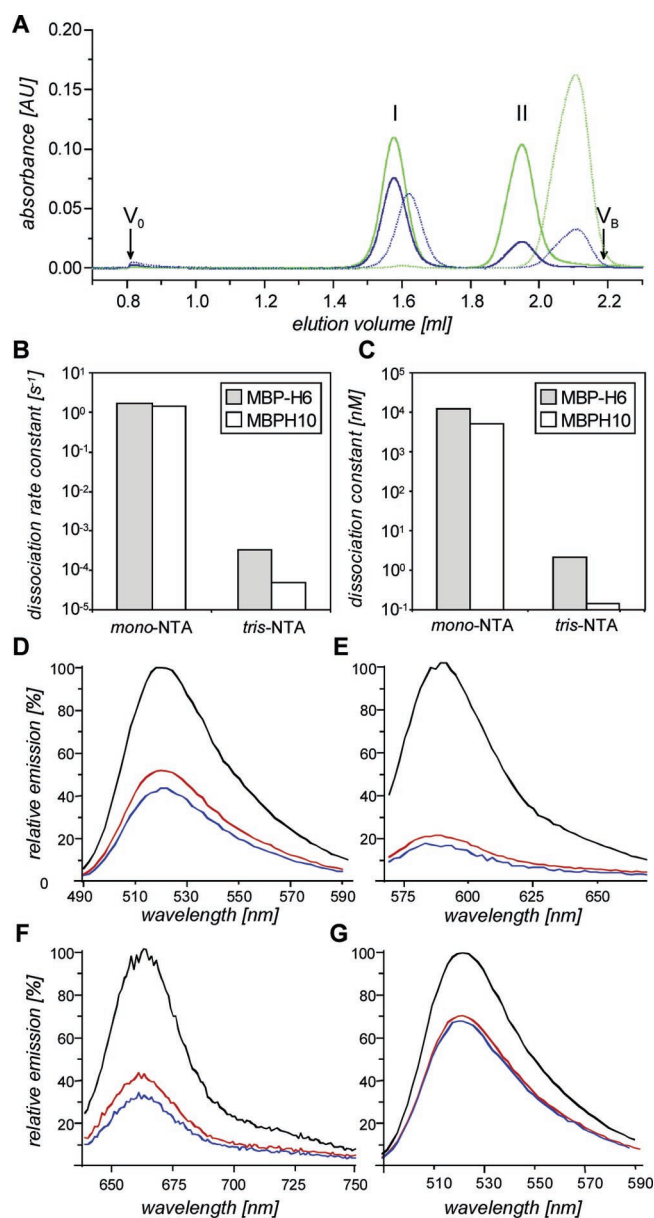
Figure 2. Stable attachment of fluorophores by tris-NTA but not mono-NTA. (A) Analytical SEC of ifnar2-H6 incubated with a 1-fold excess of OG_{488} mono-NTA (dotted line) and OG_{488} tris-NTA (solid line). Elution was monitored at 280 nm (blue) and 490 nm (green). The peaks obtained for the protein and the free conjugate are marked with I and II, respectively. The exclusion volume V_0 and the bed volume V_B are indicated by arrows. Identical labeling efficiencies and complex stabilities as for OG_{488} tris-NTA were obtained for AT_{565} tris-NTA and for FEW_{646} tris-NTA. (B) Dissociation rate constant determined for the interaction of mono-NTA and tris-NTA with MBP-H6 and MBP-H10 by monitoring fluorescence dequenching. (C) Equilibrium dissociation constants calculated from the association and dissociation rate constants, which were determined by time-resolved fluorescence measurements using OG_{488} MBP-H10 and OG_{488} MBP-H6. Fluorescence emission spectra of OG_{488} tris-NTA (D), AT_{565} tris-NTA (E), FEW_{646} tris-NTA (F), and OG_{488} -OEGtris-NTA (G). Spectra are shown for the conjugates loaded with Ni(II) ions (red), after attachment to ifnar2-H10 (blue), and after removing the Ni(II) ions with EDTA (black).
